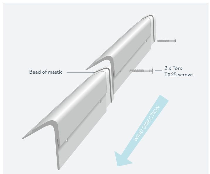
Continuously ventilated monopitch ridge
