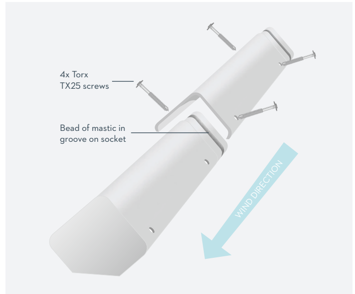
Continuously ventilated/Universal/plain angle ridge
