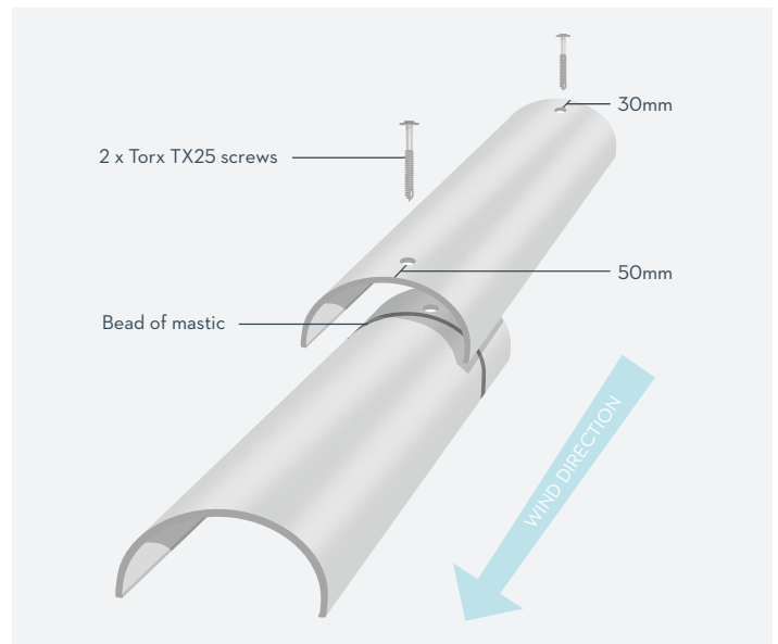
Half round/conic ridges
